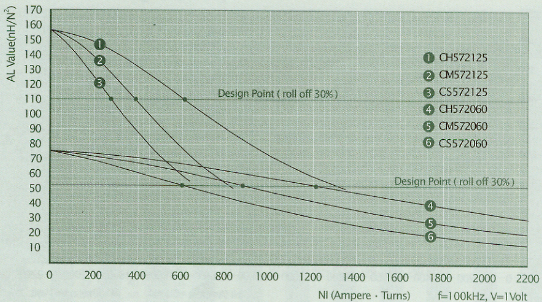
AL vs NI Curve (60 \mu , 125 \mu )
